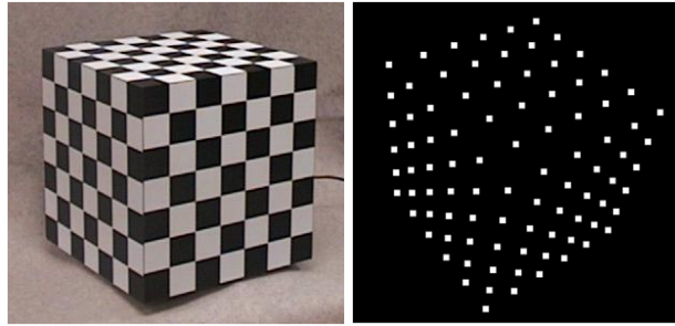
Figure 3: Calibration box and detections of corner points.
